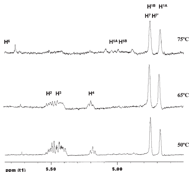
Figure 6. 1 H NMR olefinic region (400 MHz, 1,1,2,2-tetrachloroethane- d 2 , 100°C, Ref. C 2 HDCI 4 at 5.95 ppm) of iPP from rac -Et(Ind) 2 ZrCl 2 /MAO polymerized at approximately M = 1 mol/L and temperatures 50, 65 and 75°C (runs 2, 7 and 12 in Table 1).
